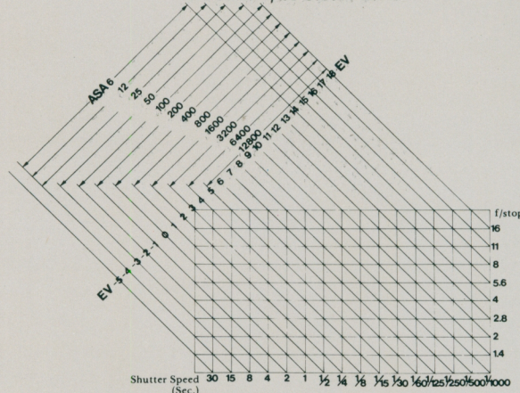
AE Range of Silicon Photocell at Various ASAs FD50mm f/1.4 S.S.C. Lens
