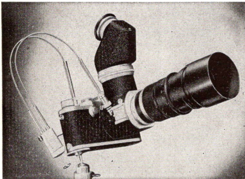
Leica IIIIf with Telyt 200mm Lens, Cat. No. 11,065 and Magnifier, Cat. No. 16,725
