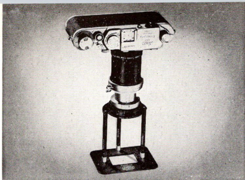
Auxiliary Reproduction Device, Cat. No. 16,515
