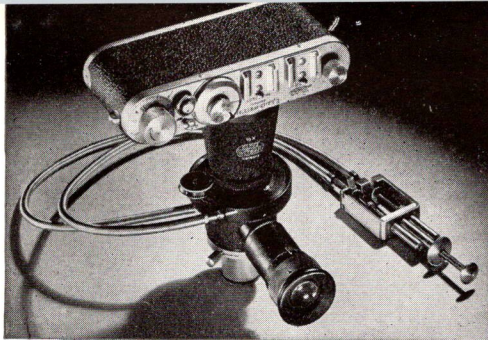
Micro Ibsor, Cat. No. 17,000 with Double Release, Cat. No. 17,010
