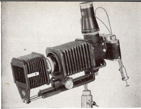
Bellows Focusing Device, Cat. No. 16,555 With Bellows Sunshade, Cat. No. 16,565 and Reflex Housing, Cat. No. 11,055
