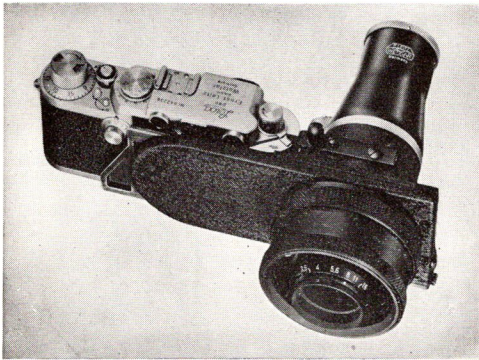
Leica IIIIf with Focaslide, Cat. No. 16,605, Diaphragm Ring, Cat. No. 16,620, Helical Mount, Cat. No. 16,610 and Magnifier, Cat. No. 16,625
