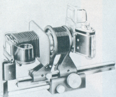
Special duplicating setup for making copies of color and black-and-white transparencies
