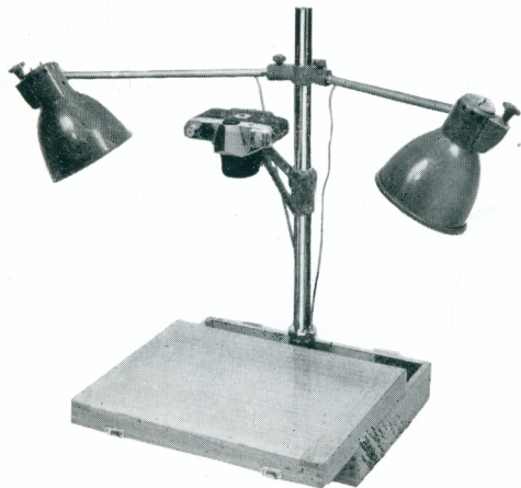
Copying Unit
