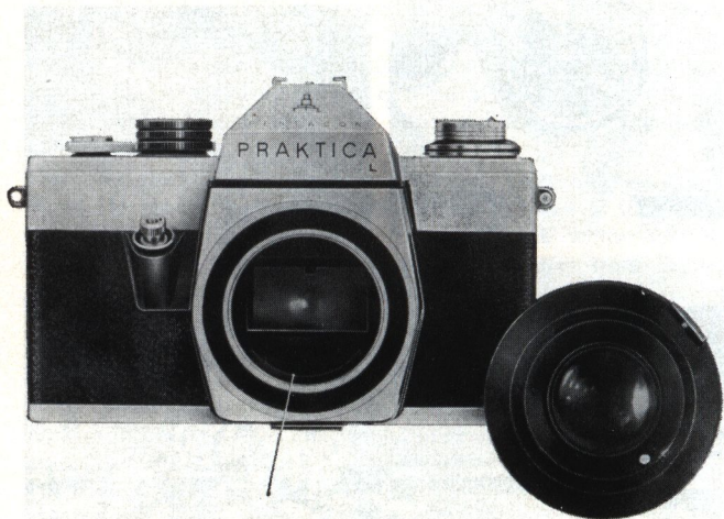
Swing-in-mechanism for automatic diaphragm
