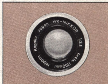
Nikkor 4" f3.5 lens
