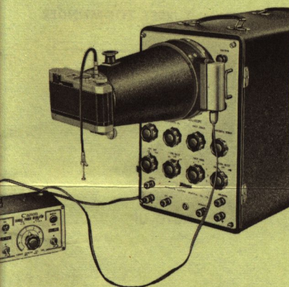
PHOTO-OSCILLOSCOPE UNITS
