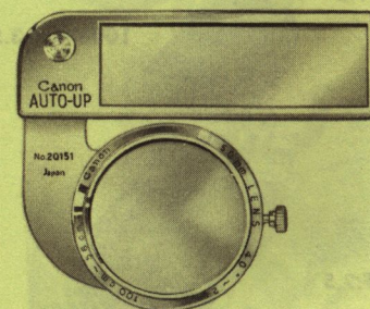
AUTO-UP
