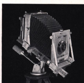
When shooting downward, linear perspective may be altered by tilting both lens and film backward to create parallelism of vertical lines.
