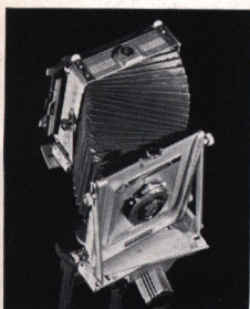
Great flexibility of both front and back permits almost unlimited combinations of adjustments of lens and film.
