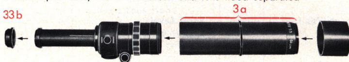
The 640 mm lens head (No. 3a) takes the place of the 400 mm lens cell
