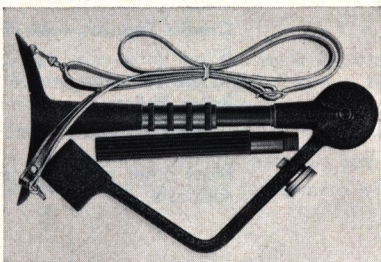
5 PISTOCK folded, measures less than 10 x 5 x 1 1/4"
