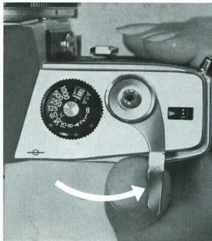
2. Advance lever
