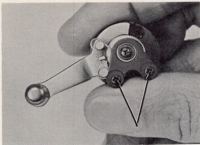
13. Remove the two bearing plate screws, washers, and the bearing plate (with late style key assembly it will be necessary to remove the wind post nut to lift out the bearing plate).
