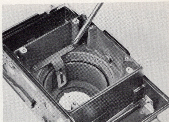
26. Adjust the free side of the tube guides to remove play on focus barrel pins. Lubricate with grease No. 7101, or equivalent. Replace the tube guides in the case and align them to allow the focus ring to revolve through the entire range with no binding.
