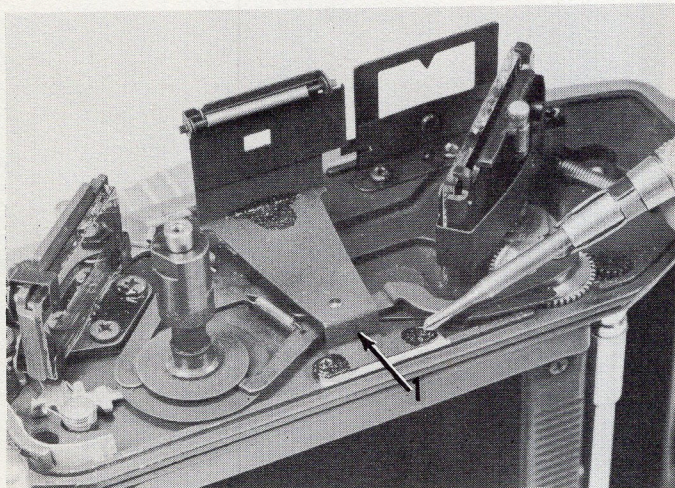
47. Replace the parallax frame assembly. Increase the tension of the assembly, if necessary, by reforming it at the point indicated by arrow 1. Too much tension will cause horizontal movement of the frame.
