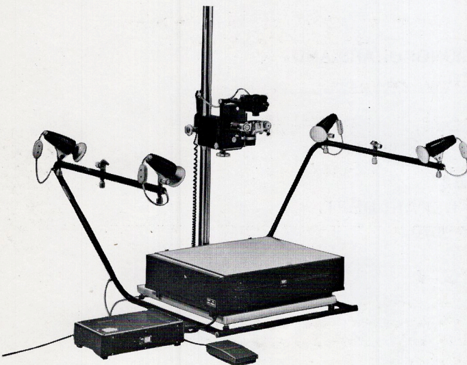
REPROPHOT 2 with floodlamp holders, flashgun brackets control box with foot switch and light box.
