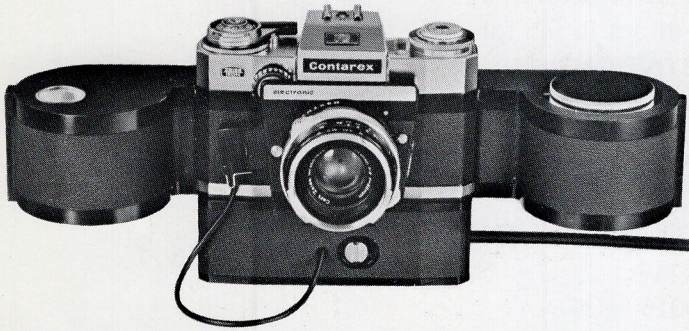
CONTAREX SE w/motor and 55 foot magazine
