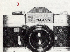
ALPA 9d w/coupled meter ALPA 6c w/uncoupled meter ALPA 6b, 5b, 8b (45° viewing)
