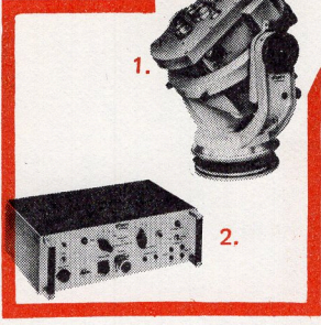
ROBOT HIGH SPEED PHOTOGRAMMETRIC CAMERA (70MM)
