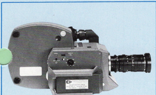
GSMO shown with Angenieux 17.5-70mm zoom lens and 120m (400') cassette-type coaxial magazine.
