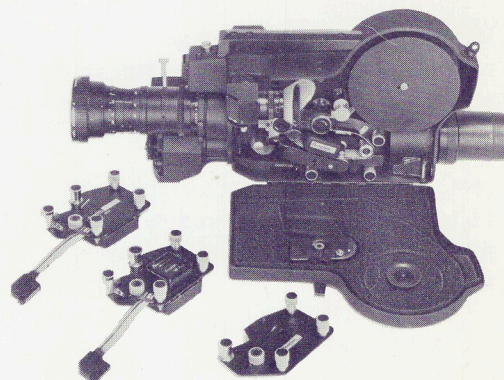
Beaulieu "News 16" camera shown together with selection of interchangeable sound module units.
