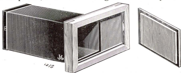
The "Ticka" Postcard Attachment. With this device on a "Ticka" Printing Box you can print on full size postcards from your negatives
