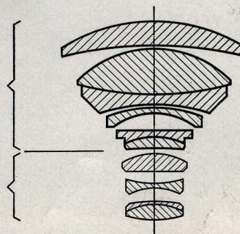
Tele attachment lens combined with 45mm Tessar lens of camera
