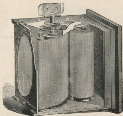
FIG. 4.--THE KODAK ROLL HOLDER.
