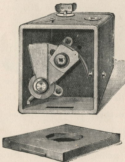
FIG. 3.--THE KODAK SHUTTER AND LENS.
